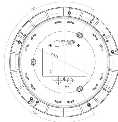
Dimension Drawing 2
